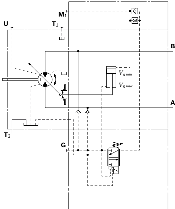
▼ Circuit diagram HA1.U1, HA1.U2
