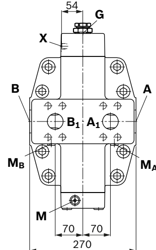
15 SAE working ports A and B lateral, opposite, A 1 and B 1 at rear
